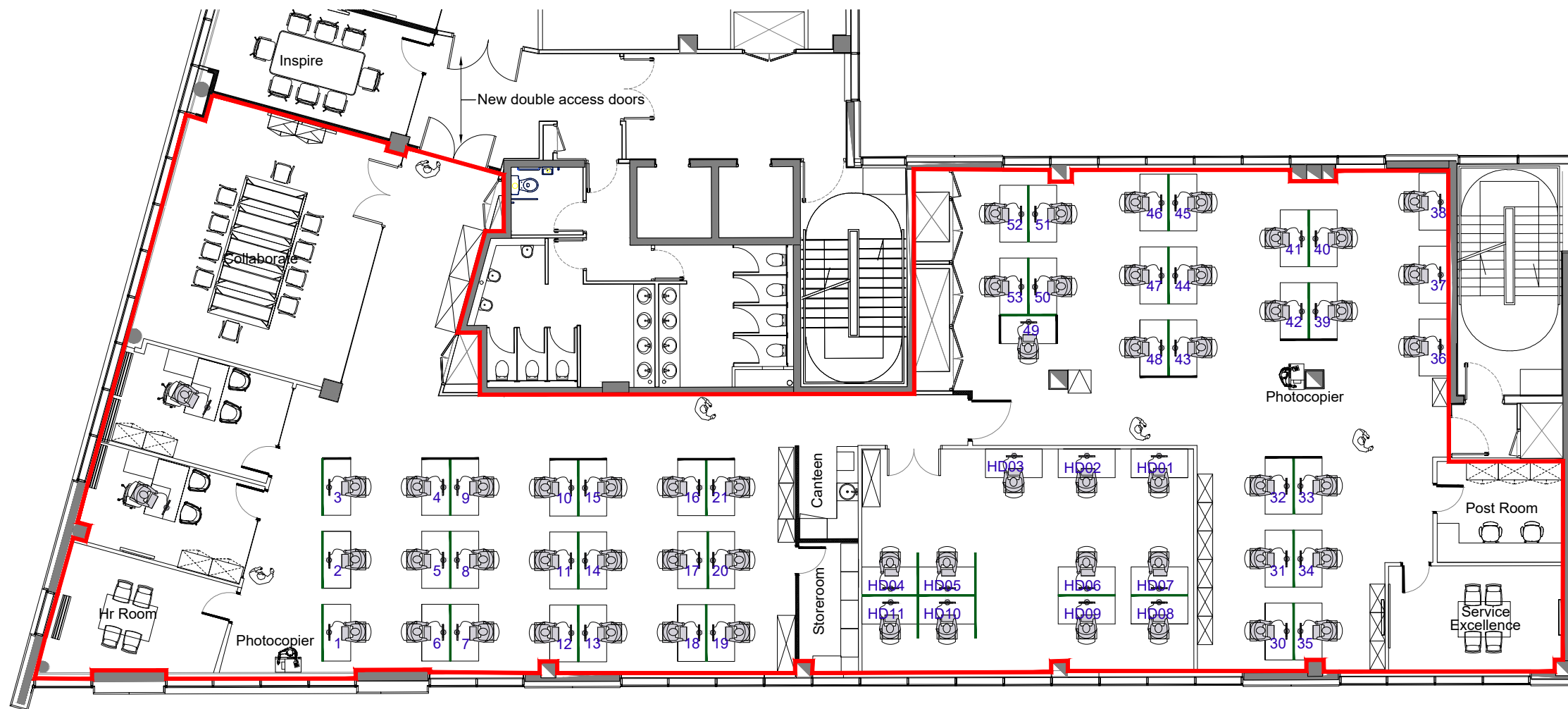
Indicative 2nd Floor Plan Rev B 14.04.2023
